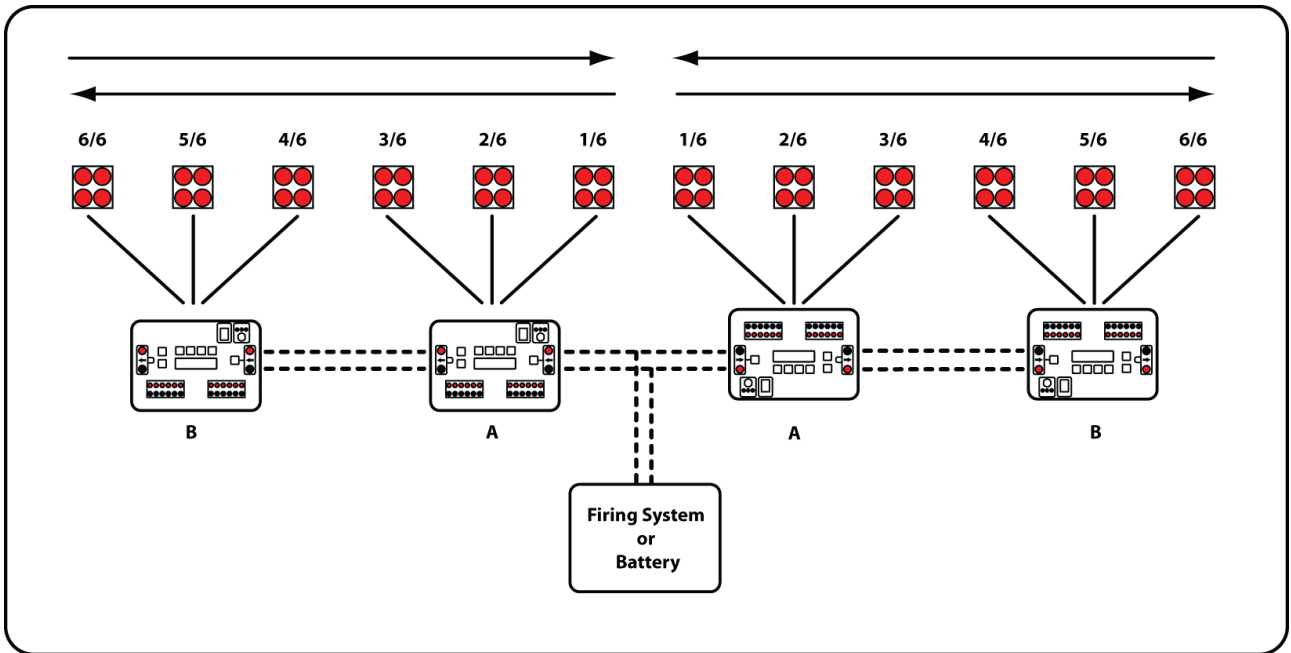
Illustration 4: Sweep Mode [Centre > Out]
